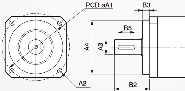
減速機出力法蘭 Output Flange of Reducer:
