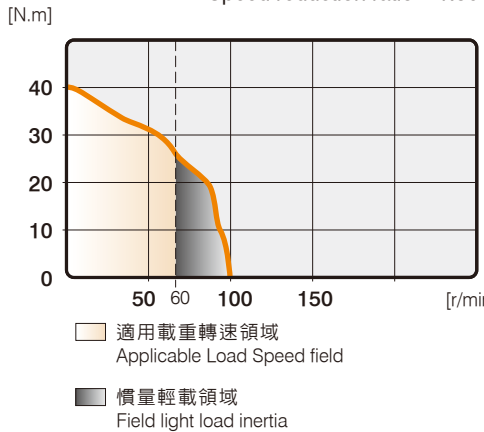
85型步進馬達定置 減速比 = 1:30 85 TYPE STEPPING MOTOR RATING Speed reduction ratio = 1:30
