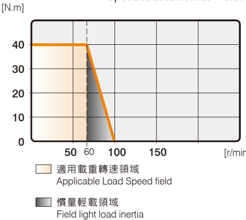
750W伺服馬達定置 減速比 = 1:30 750W SERVO MOTOR RATING Speed reduction ratio = 1:30
