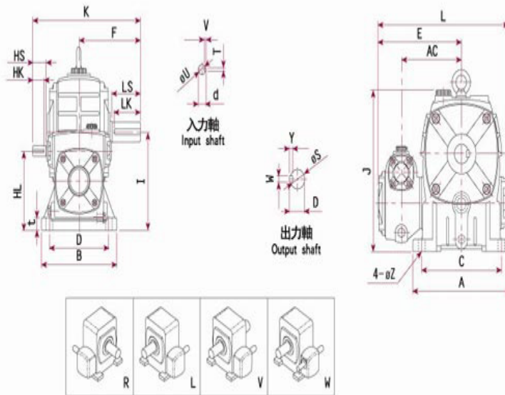
軸向選擇 Shaft Direction
