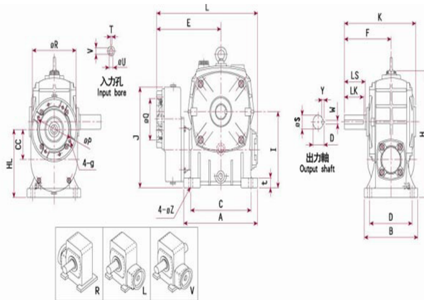
軸向選擇 Shaft Direction
